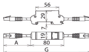
Dimension drawing DPA M CAT6 RJ45S 48
