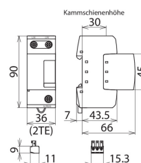
Dimension drawing DVA CSP 1P 255 FM
